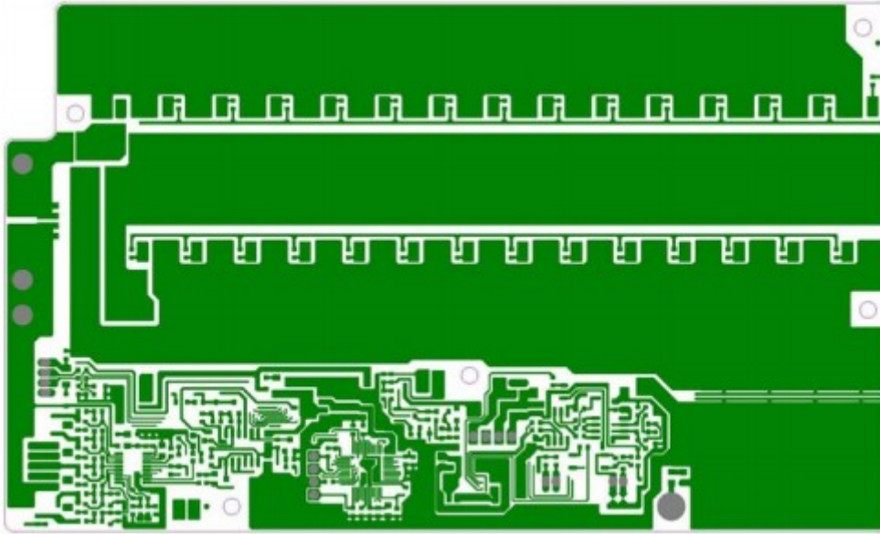
Top layer routing drawing
