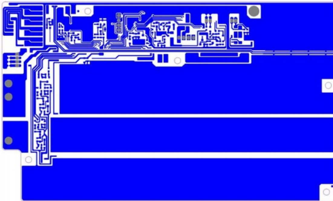
Bottom layer routing drawing
