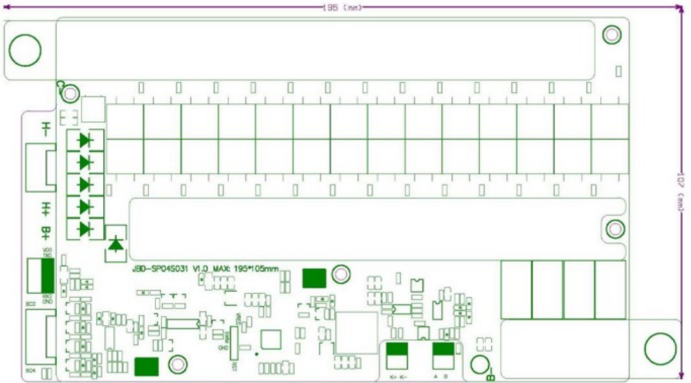
Border dimension drawing
